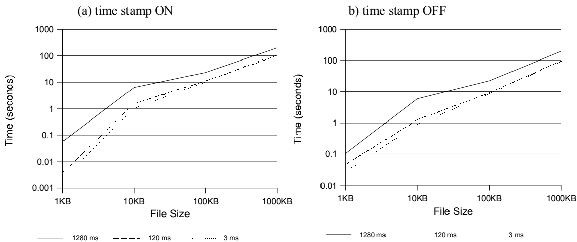
Figure 12 – Effect of time stamps on throughput for the fp protocol using the Vegas congestion control as a function of link delay for asymmetric links.
