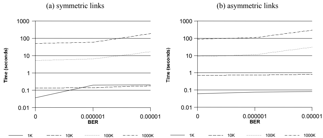
Figure 2 – Baseline ftp experiment results for symmetric and asymmetric links as a function of file size and link BER.
