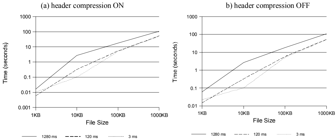
Figure 15 – Effect of header compression on throughput for the ftp protocol as a function of link delay for symmetric links.
