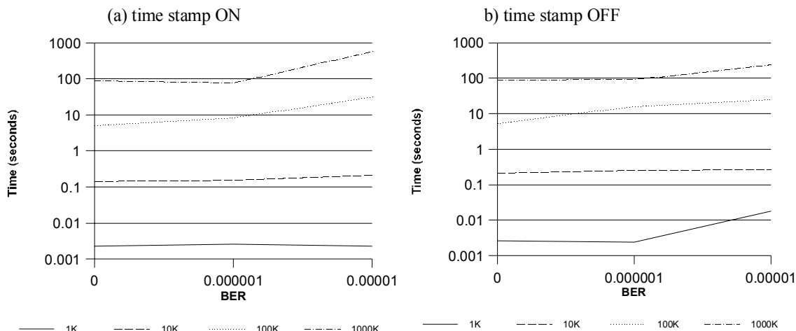
Figure 7 – Time stamp effect on throughput for the fp protocol using the Vegas congestion control on symmetric links as a function of file size and link BER.
