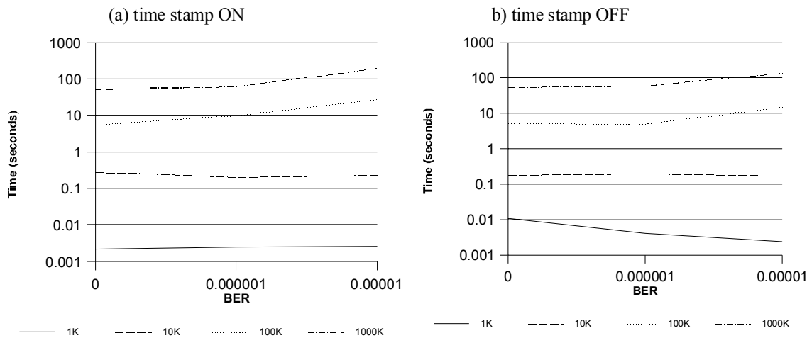
Figure 5 – Time stamp effect on throughput for the fp protocol using the VJ congestion control on symmetric links as a function of file size and BER.
