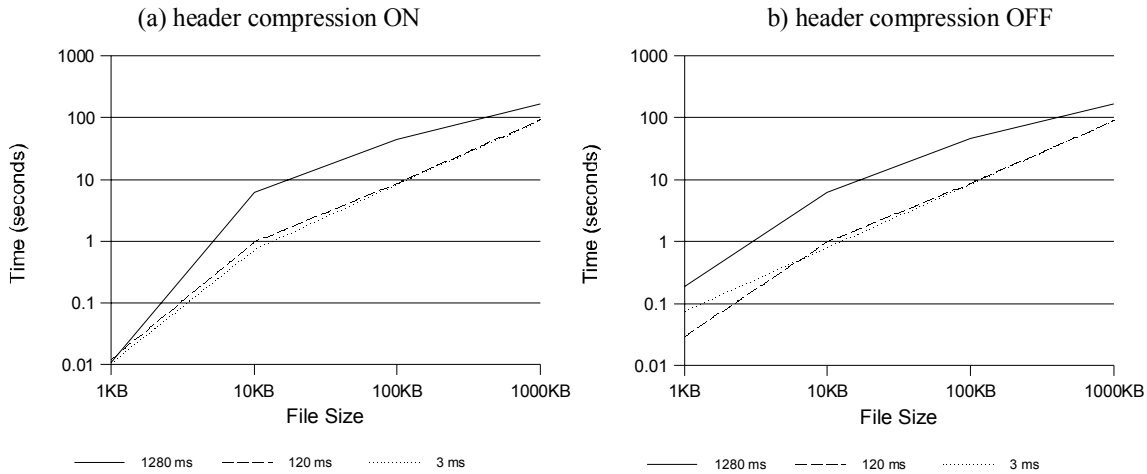
Figure 16 – Effect of header compression on throughput for the ftp protocol as a function of link delay for asymmetric links.
