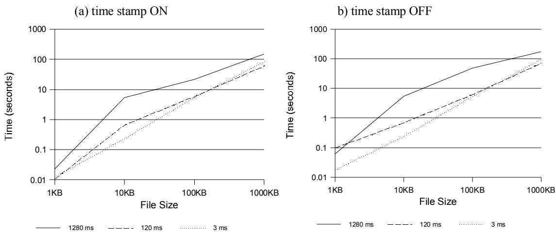
Figure 11 – Effect of time stamps on throughput for the fp protocol using the Vegas congestion control as a function of link delay for symmetric links.
