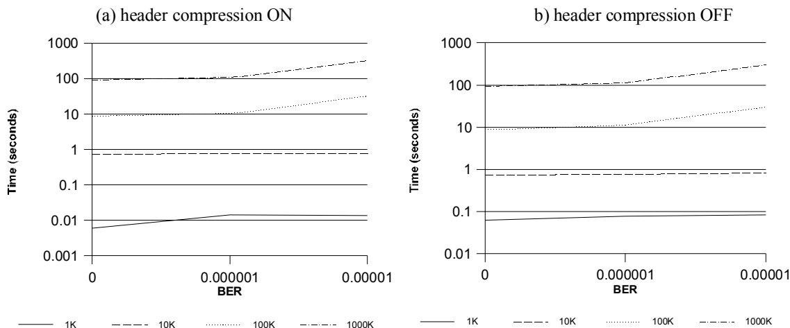
Figure 14 – Header compression effect on throughput for the ftp protocol on asymmetric links as a function of file size and link BER.
