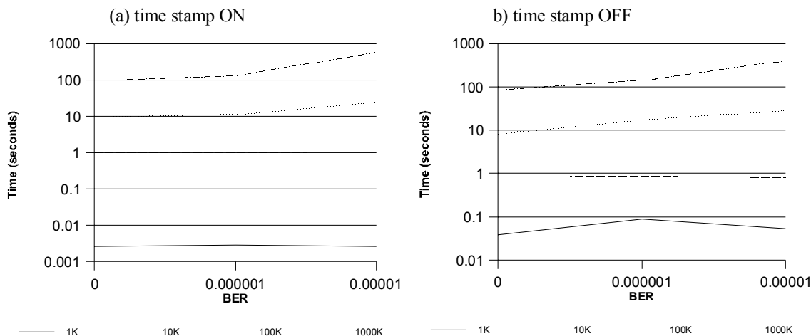
Figure 6 – Time stamp effect on throughput for the fp protocol using the VJ congestion control on asymmetric links as a function of file size and link BER.
