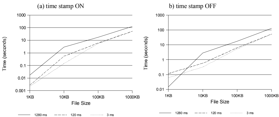
Figure 9 – Effect of time stamps on throughput for the fp protocol using the VJ congestion control as a function of link delay.
