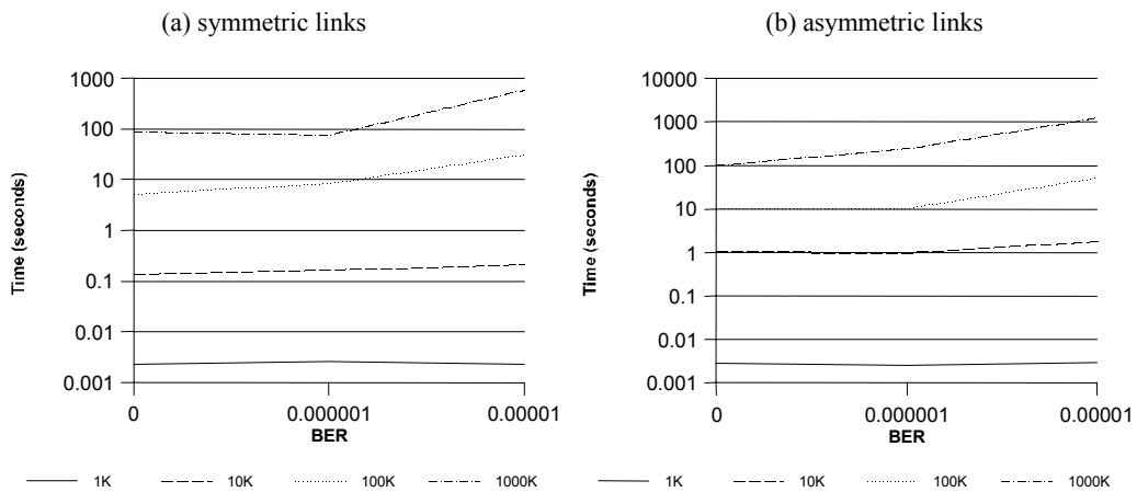
Figure 4 – Baseline fp experiment results for symmetric and asymmetric links as a function of file size and link BER and the Vegas congestion control algorithm.
