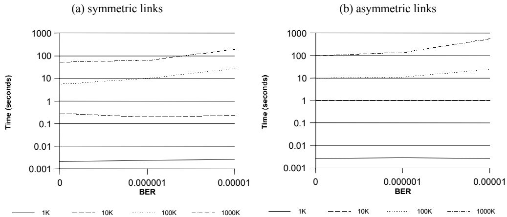
Figure 3 – Baseline fp experiment results for symmetric and asymmetric links as a function of file size and link BER.
