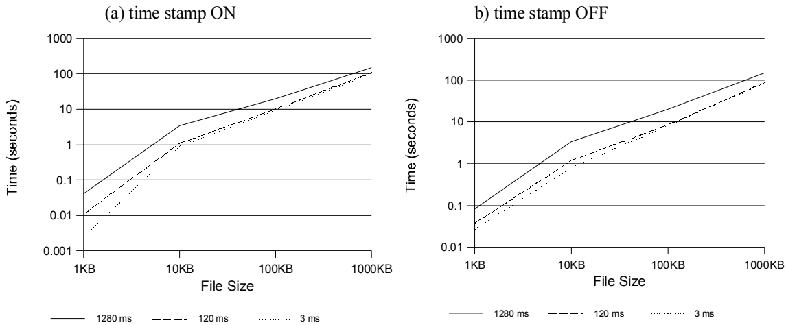
Figure 10 – Effect of time stamps on throughput for the fp protocol using the VJ congestion control as a function of link delay for asymmetric links.
